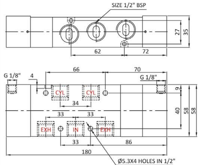
Size : 1/2" BSP (Dimensions are in mm)
